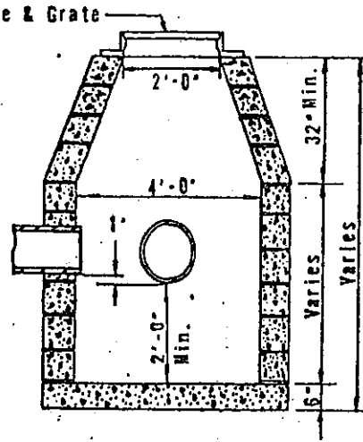
TYPE B CATCH BASIN WITH SUMP FOR MAIN DRAIN WITH SHALLOW SLOPES
