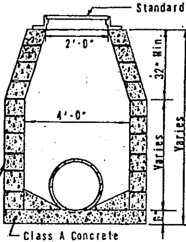
TYPE A CATCH BASIN WITHOUT SUMP FOR BRANCH DRAINS OR STEEP SLOPES
